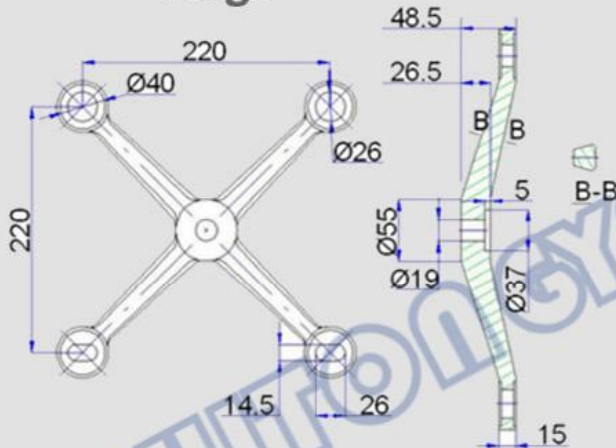
4 legs
