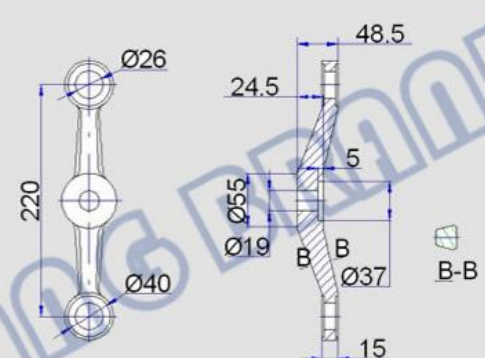
2 legs 180degree
