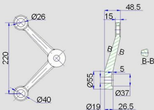
2 legs 90degree
