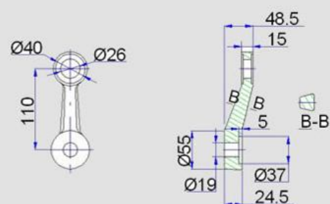
1 legs short
