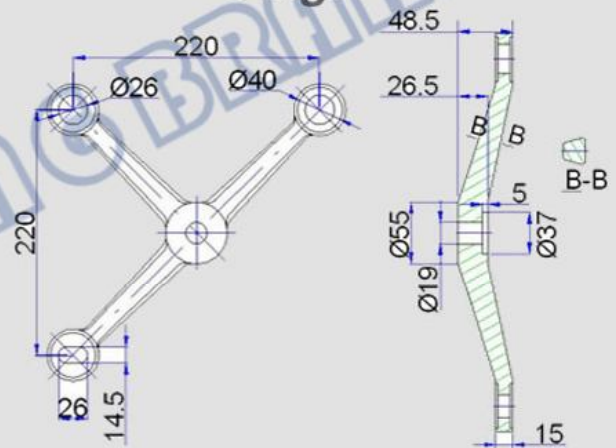
3 legs
